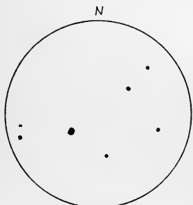
The Pleiades as seen by Good Eyes
